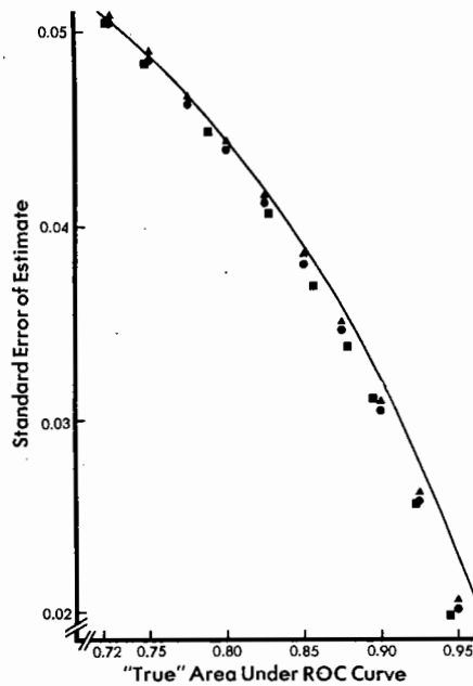
Anticipated standard error for area under ROC curve generated from different underlying distributions. Circles = Gaussian with variance ratio 1:1.5; triangles = Gaussian with variance ratio 1:0.5; squares = gamma with various degrees of freedom; solid line = negative exponential.
