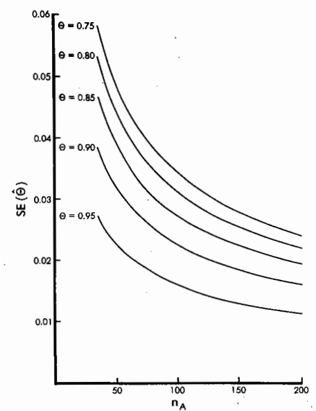
Standard error (SE) for estimated area under ROC curve ( \hat{\theta} ) in relation to sample size ( n_A = number of abnormal cases) and true area under ROC curve ( \theta ). Calculations assume an equal number ( n_N ) of normal cases.
